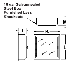
SURFACE
