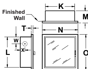
RECESSED
