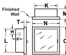
SEMI-RECESSED
