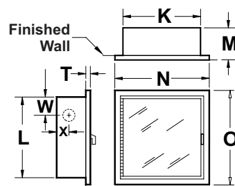
RECESSED
