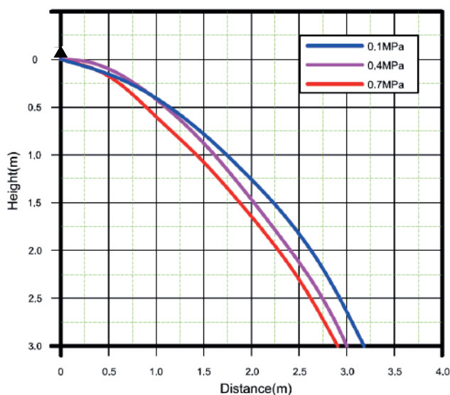
Upright (LF410/LF411)
